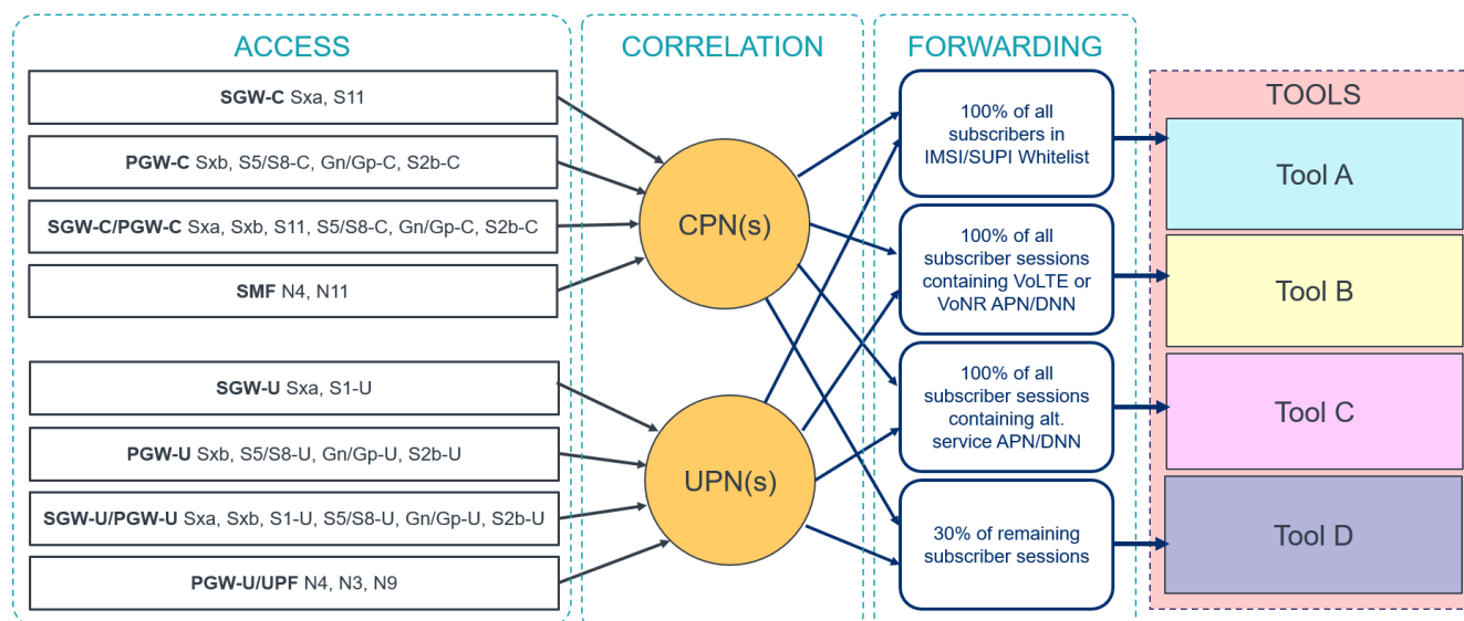
Figure 24 CUPS Traffic Visibility Solution
